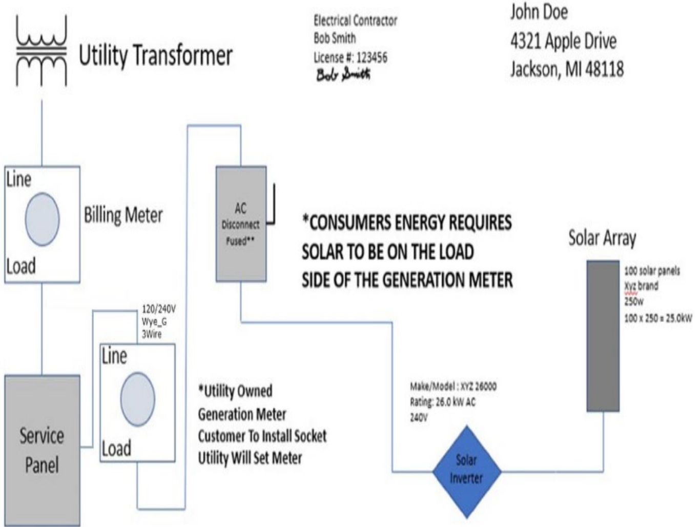
Level 2 & 3 Inverter One Line
