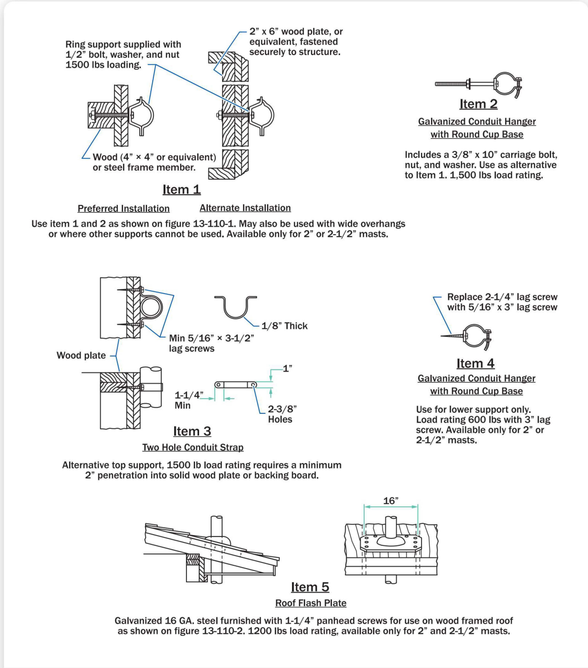
FIGURE 7 Service Mast Support Details
