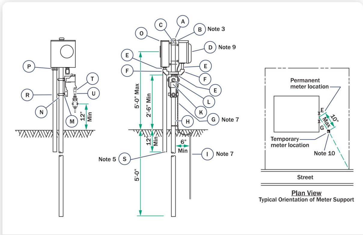
FIGURE 13 Temporary Meter Support Combination Gas & Electric (To Avoid Winter Construction) – Single Phase Meter Socket & Installations
