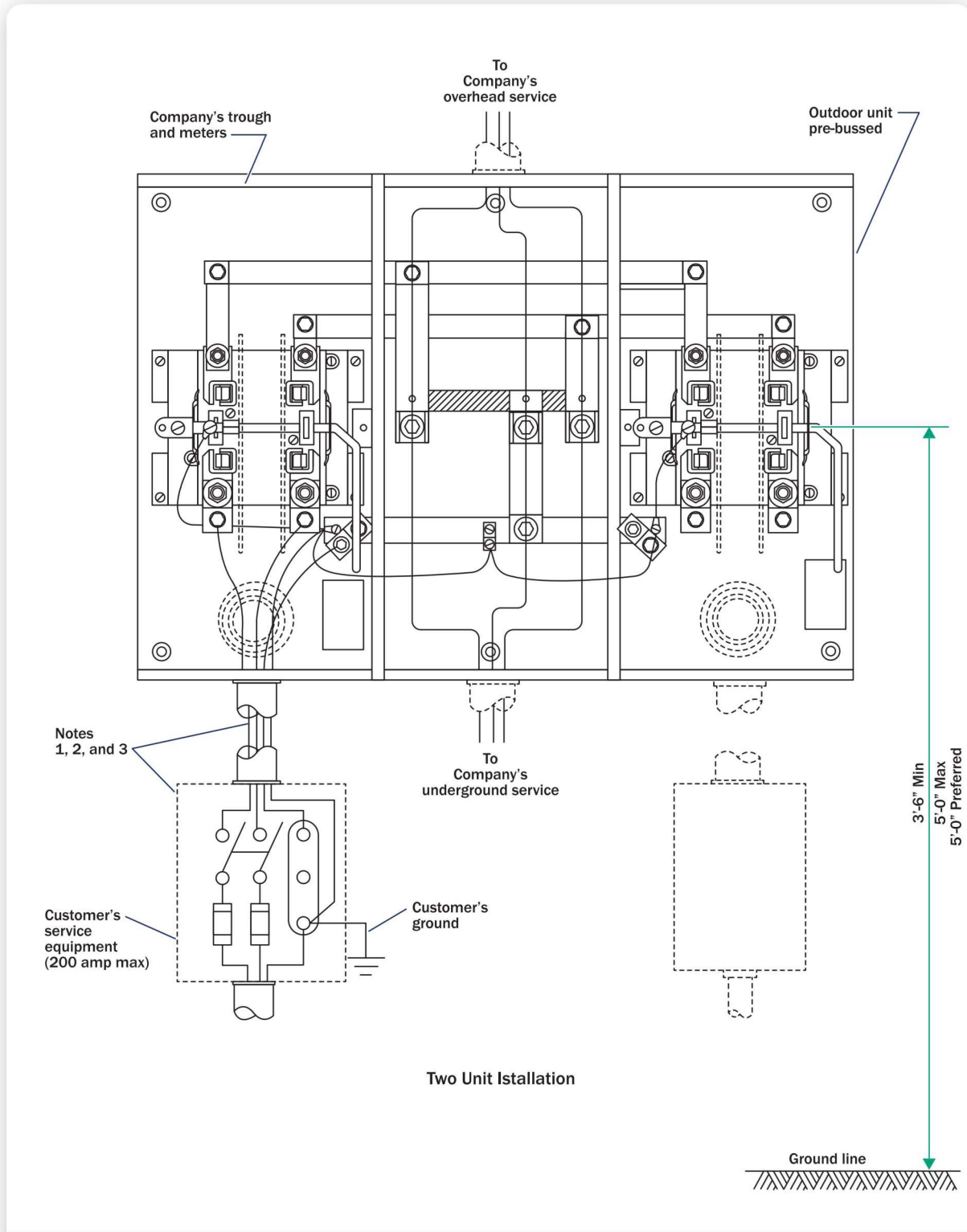
FIGURE 27 Wiring Diagram for Horizontal Grouped Meter Installations Single-Phase, 3-Wire, Two Position Self Contained Metering
