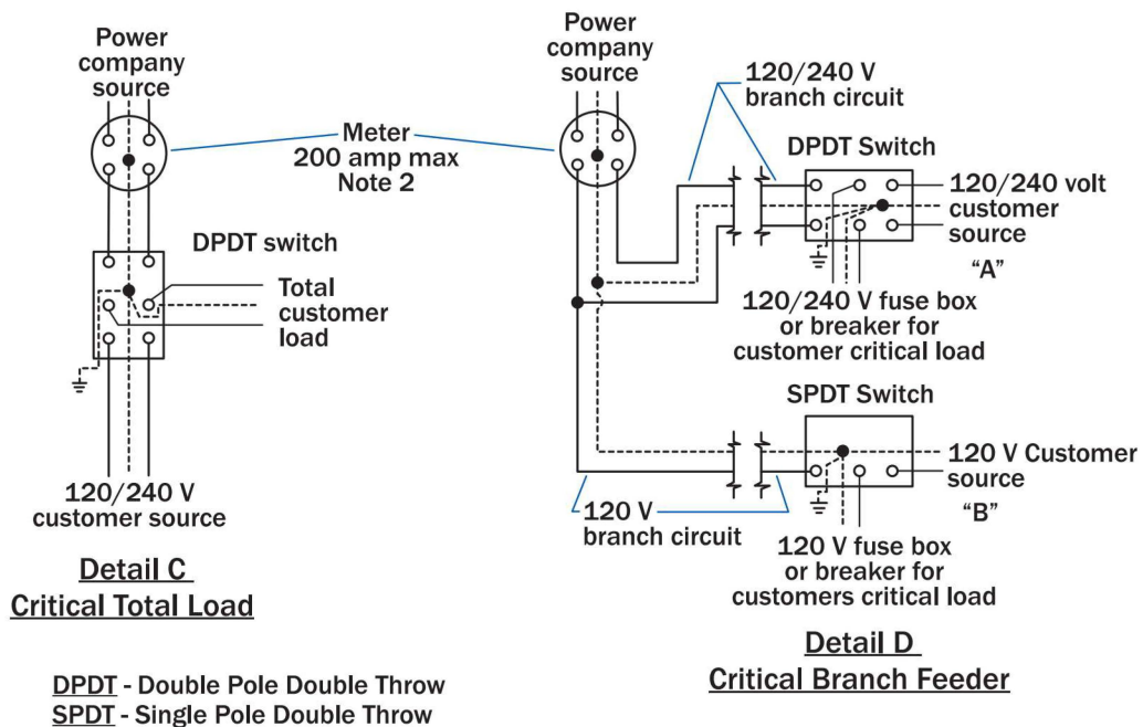
FIGURE 38 Service Switch for Use with Customer's Portable Generator Unit
