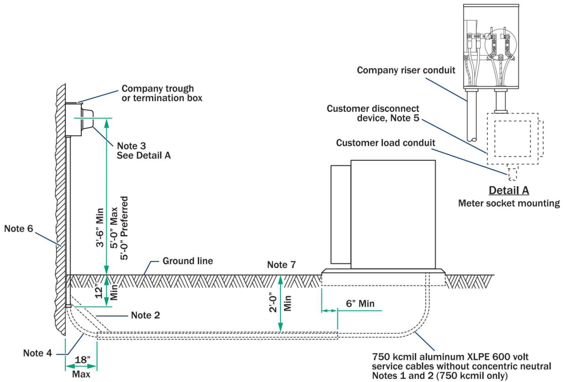
FIGURE 9 Residential Underground Service
